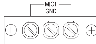
Balanced Microphone Screw Terminals
